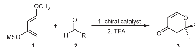
Scheme 1. The HDA between Danishefsky’s diene 1 and aldehydes 2 .
