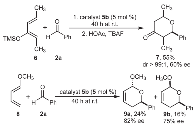
Scheme 2. Asymmetric HDA of benzaldehyde ( 2a ) with the less electron-rich dienes 6 and 8 , catalyzed by the Cr(III)-porphyrin 5b .
